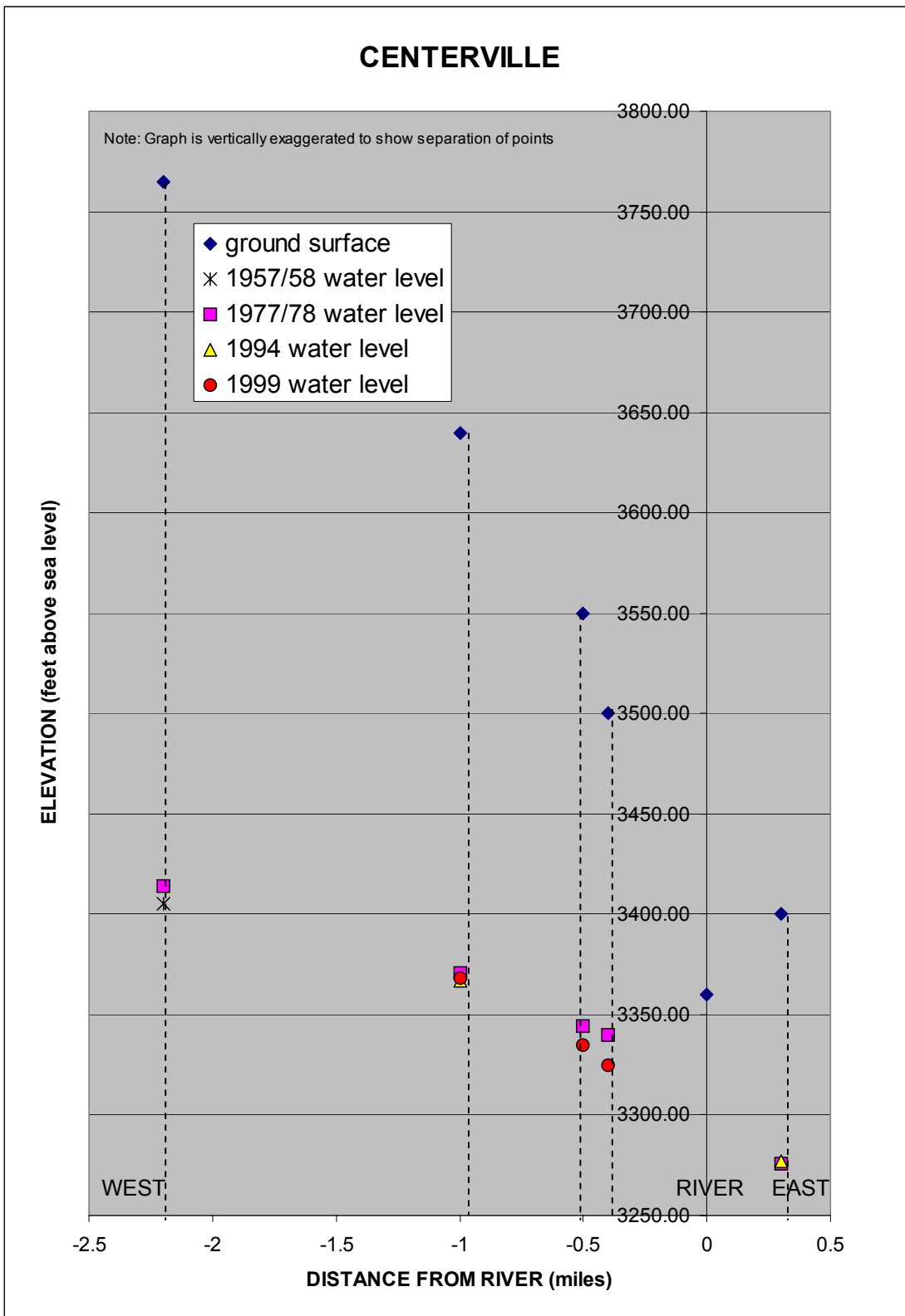
Figure C-1. Water table profile at Centerville showing water level change 1957-1999, Upper Verde Valley Riparian Area Historical Analysis.
