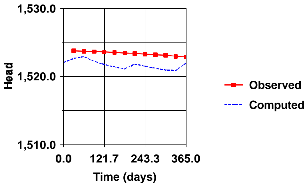
Observed vs. Simulated heads for Well 5
