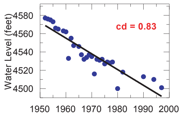
Figure 8. Hydrologic relations of water-budget analysis. The linear relations are from statistical regression analysis (Minitab 1995), and coefficients of determination (cd) are labeled. See Wirt and Hjalmarson (2000)
