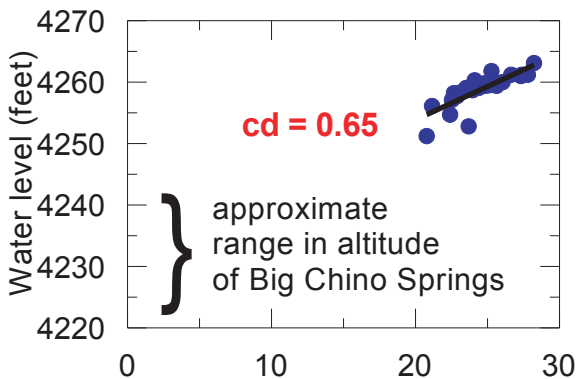
Figure 8. Hydrologic relations of water-budget analysis. The linear relations are from statistical regression analysis (Minitab 1995), and coefficients of determination (cd) are labeled. See Wirt and Hjalmarson (2000)
